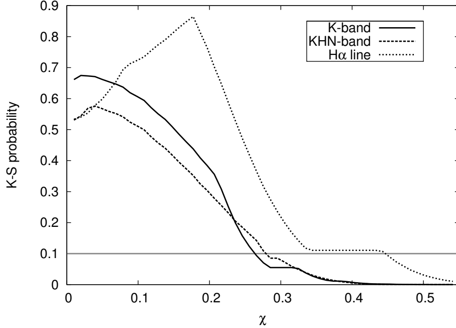
Figure 2.10: K-S test results for simulated data with single \chi values distribution for measurements in the K-band (solid line), the KHN-band (dashed line), and the H\alpha line (dotted line). The grey line represents the 90% confidence limit of the test.
