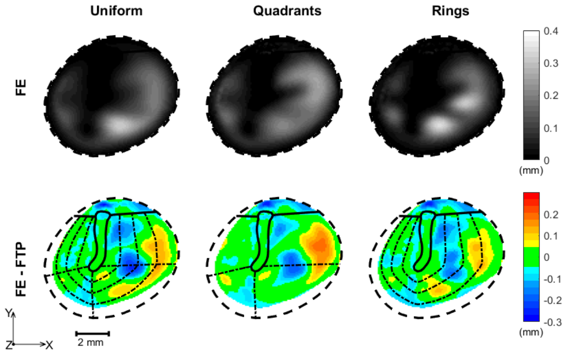
Figure 4-6: Simulated deformation patterns and error maps for sample TB3 for three types of PT partitioning: uniform (i.e., not partitioned), quadrant-based partitioning, and concentric ring-based partitioning. Top row: FE-simulated deformations. Bottom row: Error maps defined as Z^{FE,P} - Z^{FTP,P} . Anatomical directions: positive Y axis is superior direction. Positive X axis is posterior direction. The dashed boundary is the annular ring which is not observed using FTP because of the overhanging ear canal. The solid lines demarcate the manubrium and PF, and the dash-dotted lines show the partitions.
