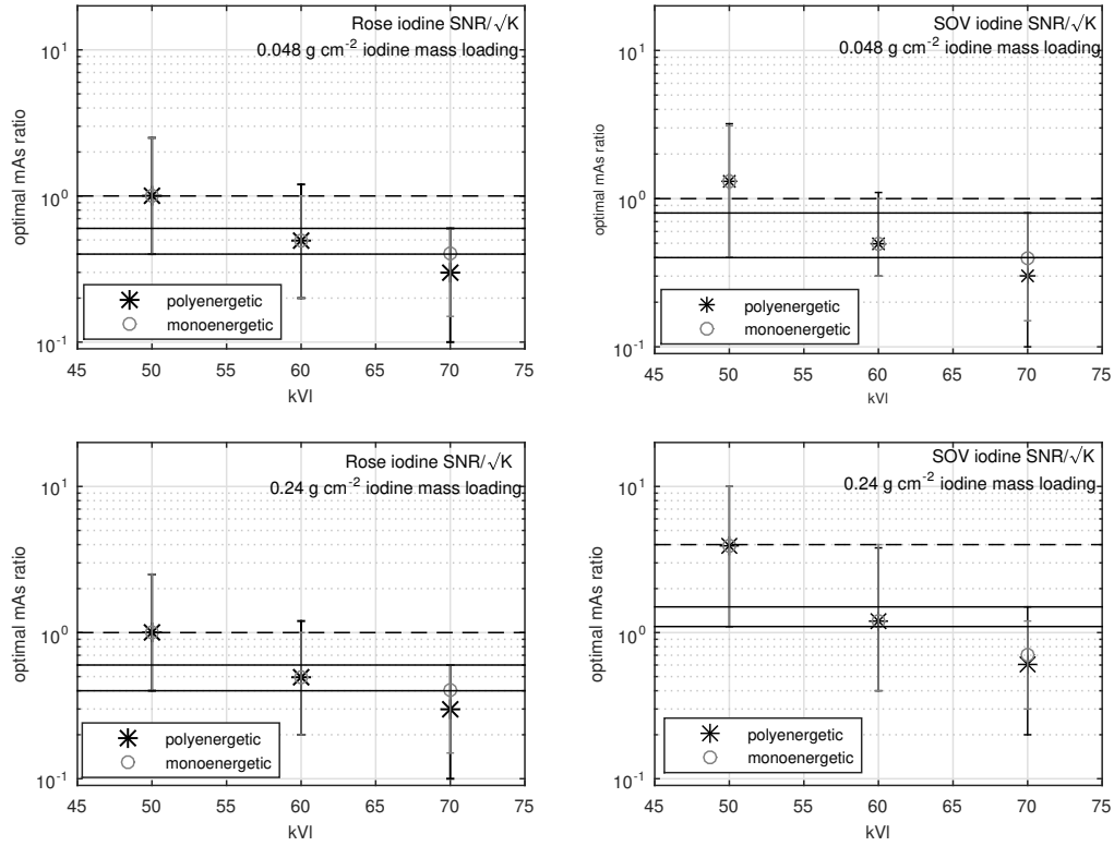
Figure 3.4.1: Optimal mAs ratio as a function of low kV that produces a maximum FOM ( \text{SNR}/\sqrt{\mathcal{K}} ) for Rose (left) and SOV (right) methods using iodine mass loadings of 0.048 \text{ g cm}^{-2} (upper) and 0.24 \text{ g cm}^{-2} (lower). The dashed line gives a near-optimal mAs ratio that is within 10% of the peak FOM at a low-kV setting of both 50 and 60 kV. The two solid lines bound a range in mAs ratio values in which the FOM is within 10% of the peak FOM for 50, 60 and 70 kV.
