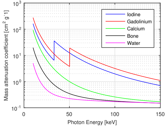
Figure 6.2.1: Mass attenuation coefficients
