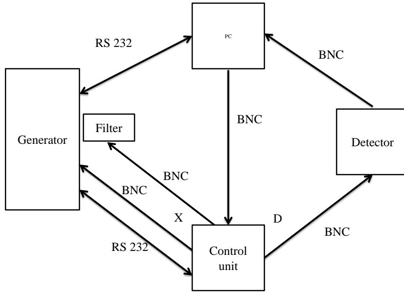
Figure 6.1.1: X-ray system design and setup showing the connection between different components and type of connection between
