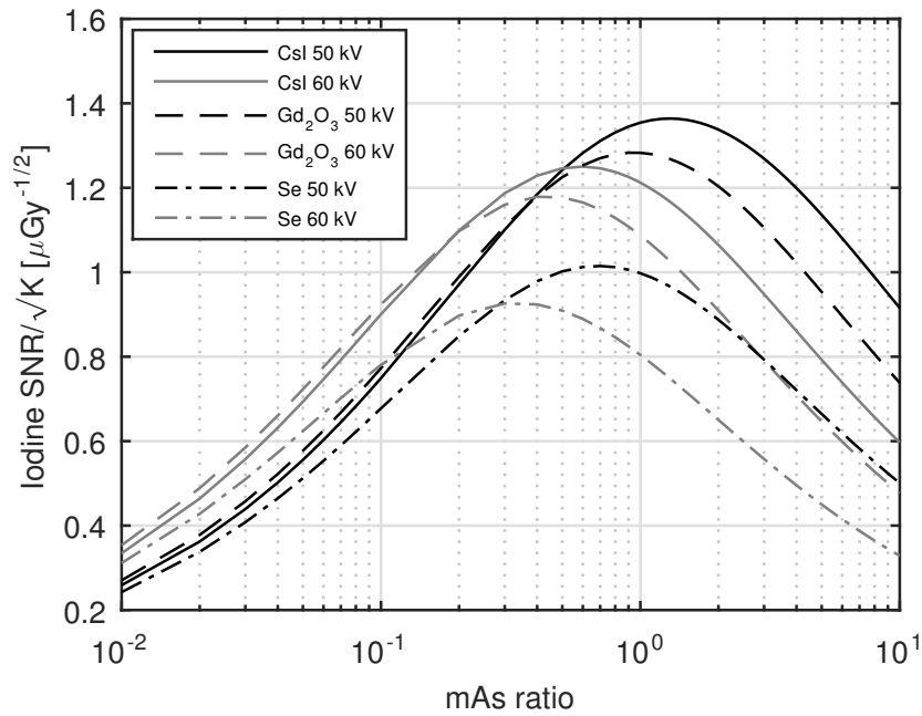
Figure 3.4.5: Theoretical polyenergetic iodine \text{SNR}/\sqrt{\mathcal{K}} as a function of mAs ratio for CsI, Se and \text{Gd}_2\text{O}_3 detector converter materials for an iodine mass loading of 0.048 \text{ g cm}^{-2} for 20 cm of water for a fixed high kV (120 kV) and low kV of 50 and 60 kV.
