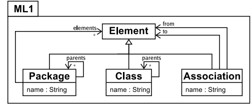
(a) The ML1 modelling language.
