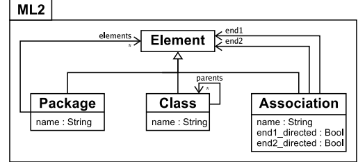
(b) The ML2 modelling language.
