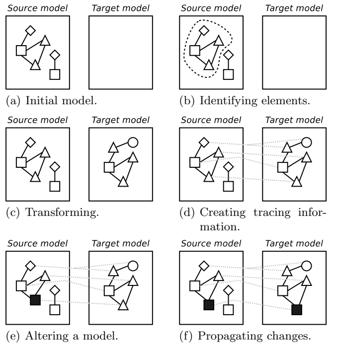
Fig. 4 Transforming a model.
