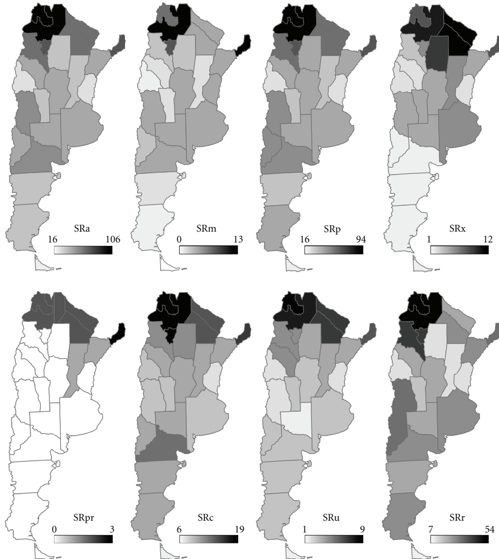
FIGURE 2: Species richness of indigenous nonvolant terrestrial mammals in each Argentinean province. SRa: all mammals; SRm: Marsupialia; SRp: Placentaria; SRx: Xenarthra; SRpr: Primates; SRC: Carnivora; SRu: Ungulates; SRR: Rodentia.
