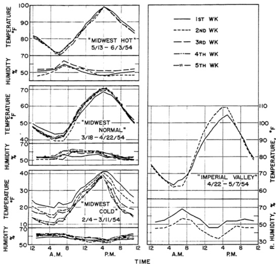
Fig. 3—Same as Fig. 2 but for the spring , 1954, period. Each curve represents the average for a week and was plotted from average data of one-hour intervals for temperature and two-hour intervals for humidity. "Midwest Cold" and "Midwest Normal" were of five weeks' duration, "Midwest Hot", three weeks', and "Imperial Valley" two weeks' duration.
