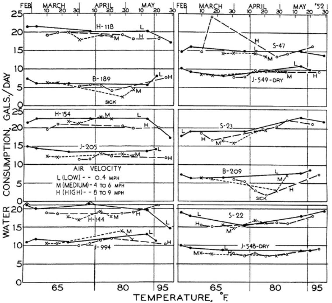
Figure 3 — Water consumption at 65°F and 80°F was slightly depressed by high air velocity.
