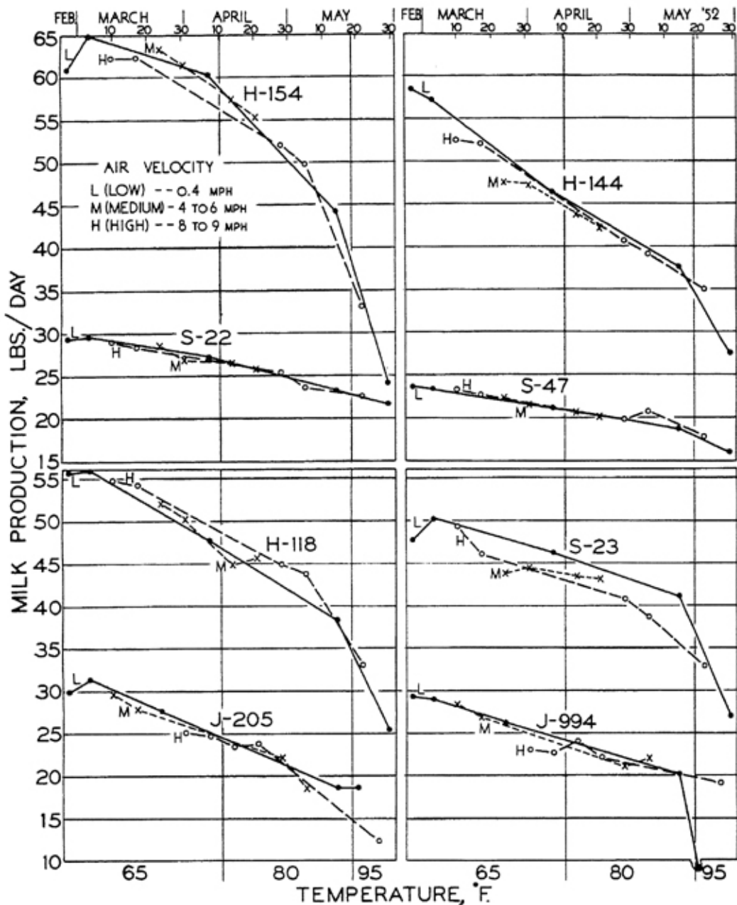
Figure 1—A comparison of the effects of low, medium, and high air velocity on milk yield at 65°, 80°, and 95°F. The slopes of the curves (due to rising temperature and advancing stage of lactation) were not affected by wind except at 95°F when the milk yield at 0.4 mph was lower than that at 9 mph in the Holsteins (H), in the highest yielding Brown Swiss (S) and in one of the two Jerseys (J).
