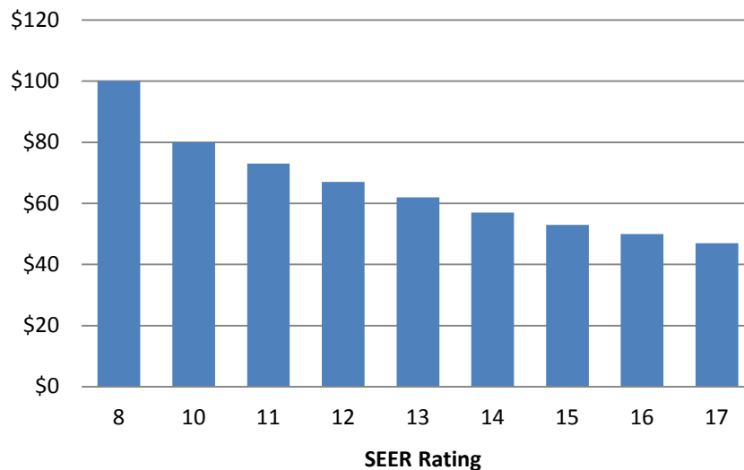
Figure 10: Impact of Efficiency (SEER Rating) on Annual Energy Costs
