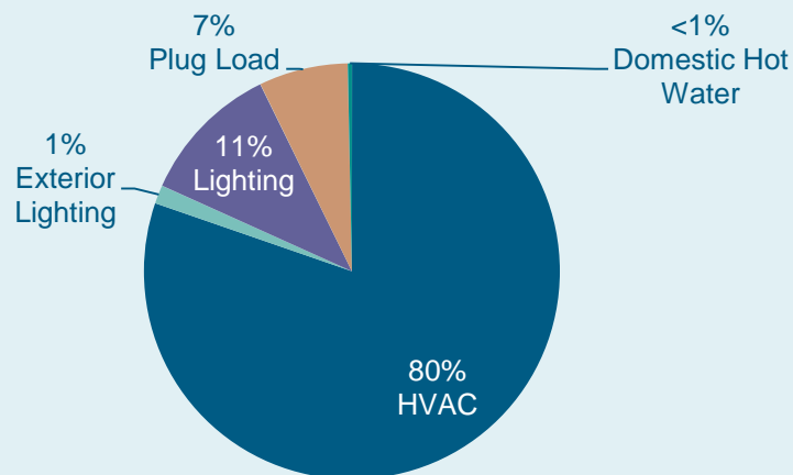
Figure 12: Average Energy End Uses for Police/Admin Buildings
