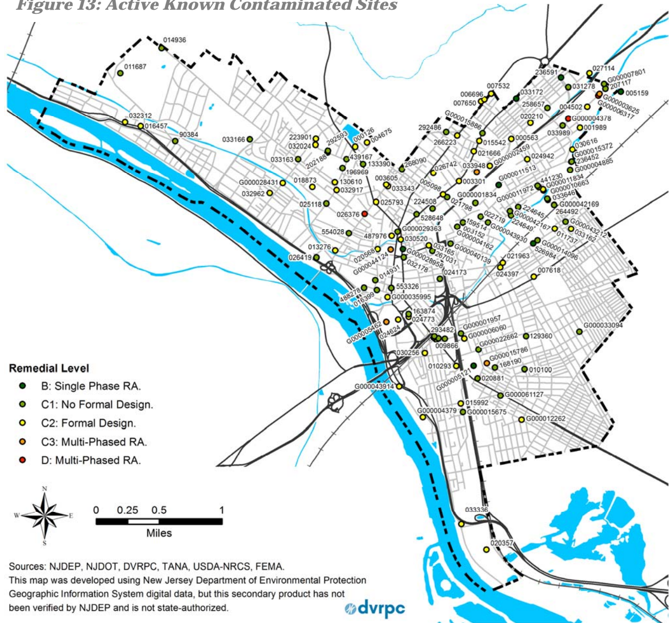
Figure 13: Active Known Contaminated Sites
