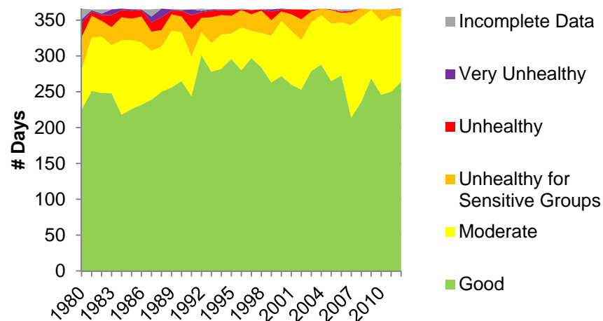
Figure 14: Air Quality Index for Trenton-Ewing CBSA, 1980–2012
