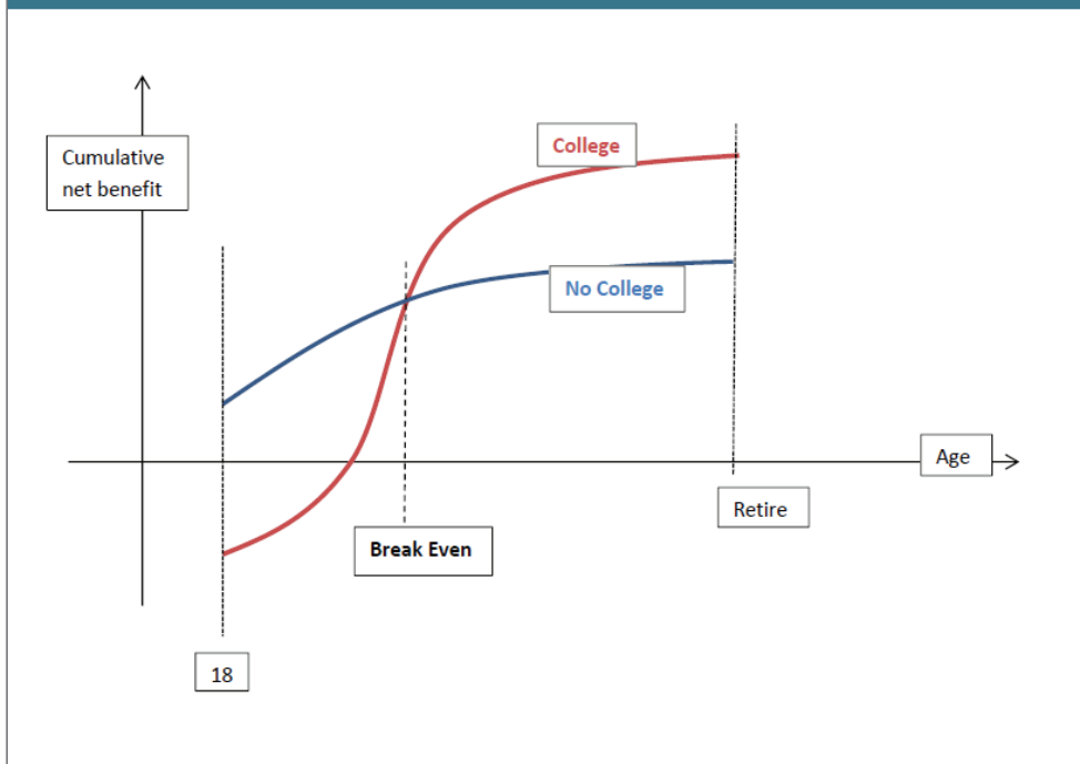
Figure 3: Break-even Age
