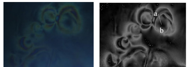
Figure 7. (a) Fringe patterns under foot loading (b) phasemap
