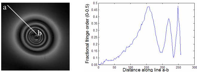
Figure 5. Phasemap under monochromatic light (a) with modified equation, (b) fractional fringe order along a-b.
