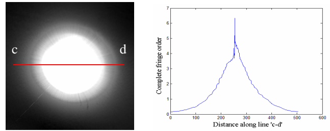
Figure 6. (a) Unwrapped phasemap with, (b) complete fringe order along 'c-d'.
