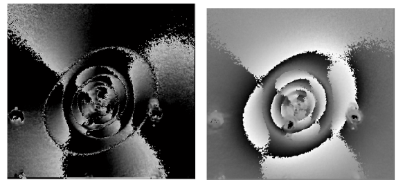
Figure 4. Phasemap using monochromatic light (a) isoclinics, (b) isochromatics
