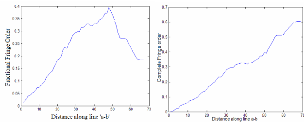
Figure 8. Fractional and complete fringe order along line 'a-b'
