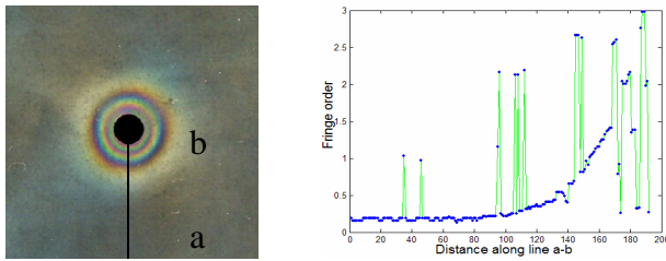
Figure 3. Fringes under unconventional loading (a) fringes due to indenter loading, (b) fringe order along line a-b.
