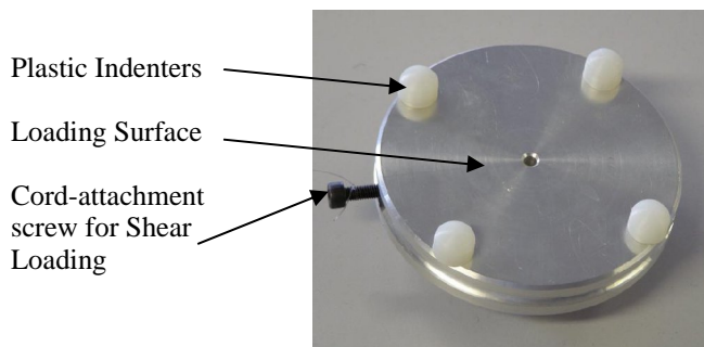
Figure 1. Loading plate with indenters
