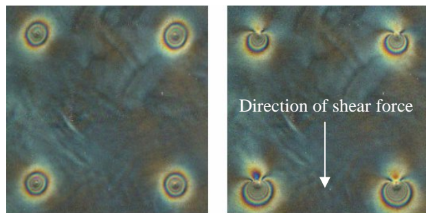
Figure 2. Fringe patterns under (a) vertical, (b) shear loads
