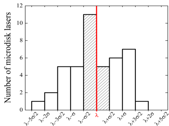
Figure 4. Wavelength distribution of 43 microdisk lasers from the same sample centered on \lambda . The patterned area shows that the peak lasing wavelength of 16 microdisk lasers is between \lambda-\sigma/2 and \lambda+\sigma/2 (with \sigma=500\text{pm} ).
