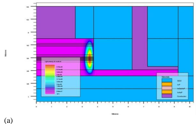
Figure 6. Schematic structure of the InP microdisk structure for two alternative epitaxial layer stacks: (a) with the epilayer structure including a tunnel junction, (b) layer structure with a regular pin junction, of which the highly absorbing contact layers are etched away at the edge.
