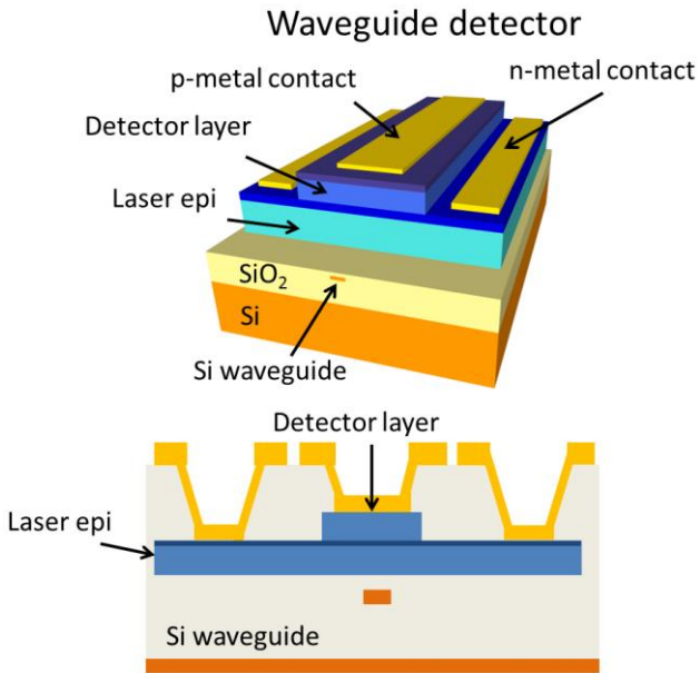
Figure 13. Schematic overview of the detector design, where (a) shows a 3D impression and (b) shows the cross section of the detector.
