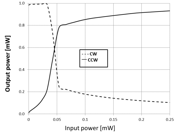
Figure 11. Static regeneration characteristic for a microdisk laser with K_2/K_1=10 .
