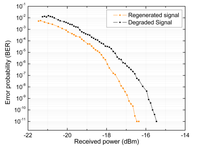
Figure 12. Measured BER curves at 10 Gb/s, before and after regeneration with a microdisk laser.
