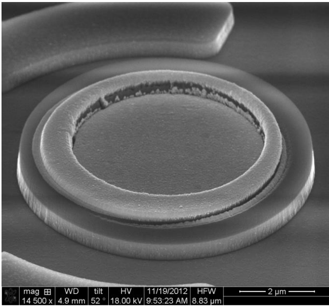
Figure 5. SEM image of an etched microdisk with a self aligned top contact. It can be seen that the Titanium-gold metal itself is misaligned, but the metal area that contacts the disk is perfectly in the center thanks to the nitride ring.
