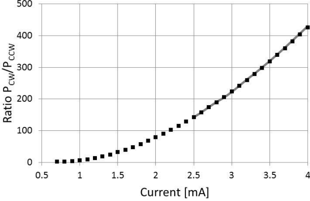
Figure 10. Ratio of power in CW and CCW modes, (■) obtained from a numerical solution of the coupled rate equations, for a microdisk laser with coupling coefficients K_1=6.36 \cdot 10^8 \text{ s}^{-1} , K_2=3.18 \cdot 10^8 \text{ s}^{-1} , and (—) obtained from expression (23). \varepsilon=10^{-18} \text{ cm}^3 .
