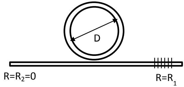
Figure 8. Schematic structure of a ring/disk laser coupled to a bus waveguide, containing a reflector on one side.
