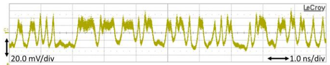
Figure 15. Large signal modulation response of the full optical link for a 10\ \text{Gb/s} 2^7-1 PRBS pattern.
