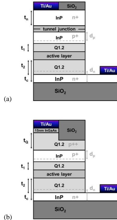
Figure 6. Schematic structure of the InP microdisk structure for two alternative epitaxial layer stacks: (a) with the epilayer structure including a tunnel junction, (b) layer structure with a regular pin junction, of which the highly absorbing contact layers are etched away at the edge.
