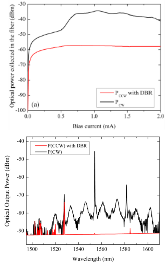
Figure 9. L-I characteristics (top) and spectrum at 1.2 mA (bottom) of a microdisk laser coupled to a waveguide with a Bragg grating on one side. The optical power is the power collected in optical fibers on both sides of the waveguide.
