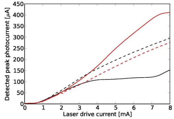
Figure 14. Current versus current plot for two different optical links (dashed and solid lines) under pulsed drive conditions. The black and red curves correspond with the left and right detector, respectively.
