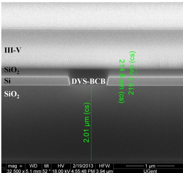
Figure 3. FIB cross-section of a device where a 100nm thick SiO 2 layer has been deposited prior to bonding with the wafer bonder. The measured total bonding thickness is 220nm and the DVS-BCB layer thickness is 120nm.
