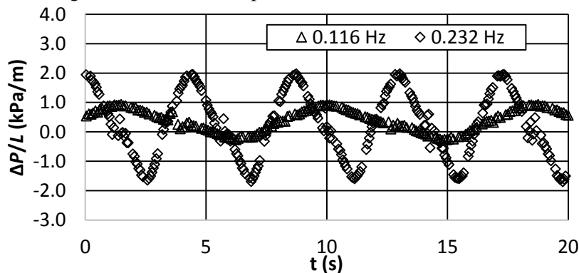
Figure 7. Pressure gradient versus time - Effect of frequency at a displacement of 97.23 mm
