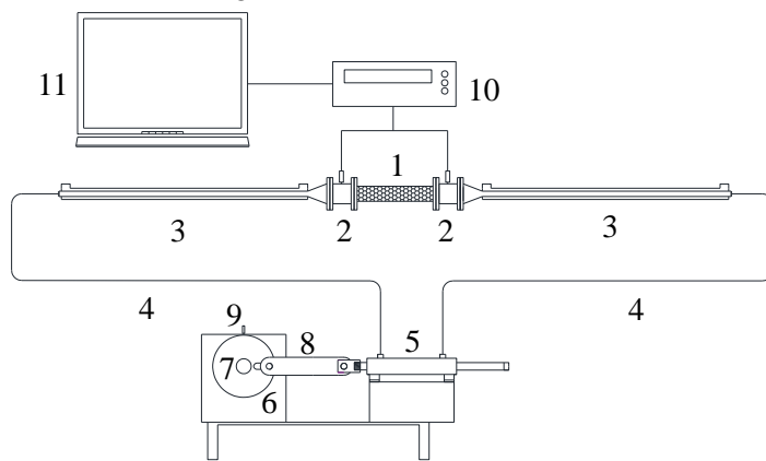
Figure 1. Schematic of the experimental setup: 1. Test Section, 2. Polyethylene tubes, 3. Steel pipes, 4. hoses, 5. Oscillation Generator, 6. Motoreductor, 7. Flywheel, 8. Crank Arm, 9. Optical sensor, 10. Data logger, 11. Computer.
