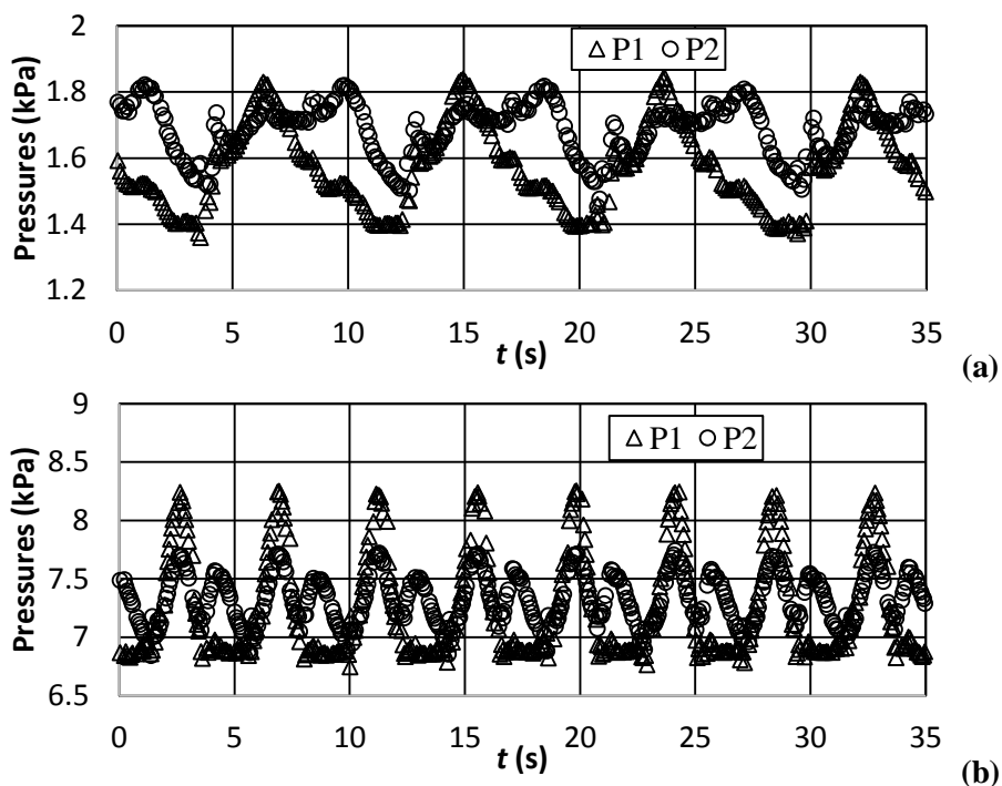
Figure 5. Temporal pressures at inlet and outlet for x_{\max} = 97.23 mm: (a) \omega = 0.116 Hz, (b) \omega = 0.232 Hz
