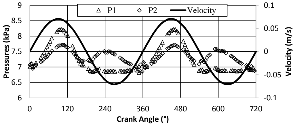
Figure 4. Temporal pressures at inlet and outlet and average flow velocity for x_{\max} = 97.23 mm: \omega = 0.232 Hz.
