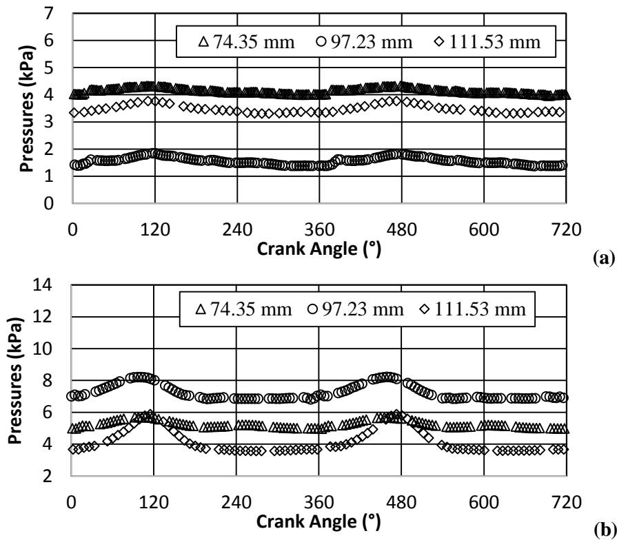
Figure 6. Temporal pressure at inlet- Effect of displacement for (a) \omega = 0.116 Hz, (b) \omega = 0.232 Hz
