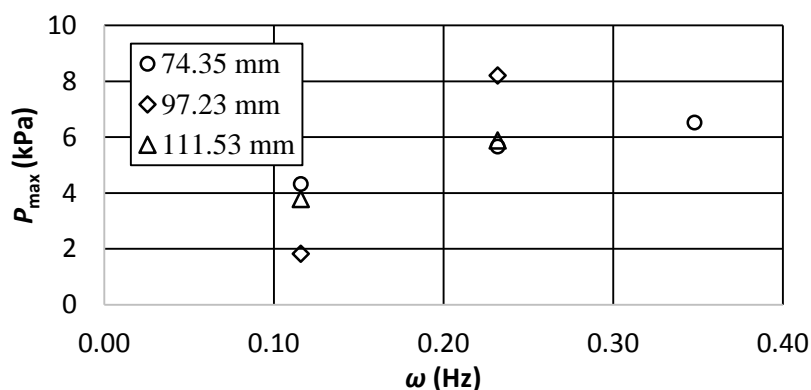
Figure 3. Inlet pressure amplitude as a function of flow frequency for different fluid displacements
