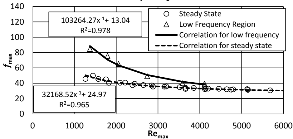
Figure 8. Friction factor versus Reynolds number for steady and oscillating flow for all flow displacements
