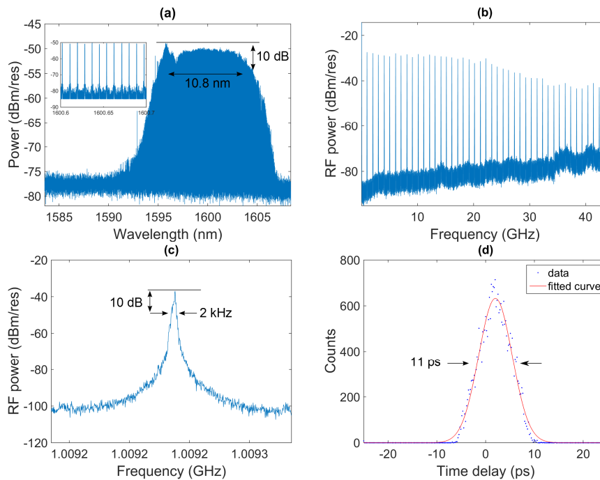
Figure 2 (a) Optical spectrum taken with a high resolution optical spectrum analyzer. The inset shows a detail of evenly spaced optical modes within the comb. (b) RF spectrum of the generated pulse train (RBW 300 KHz, VBW 10 KHz) (c) Detail of the 1 GHz RF tone (RBW 0.51 kHz, VBW 0.51 kHz) (d) Auto correlation trace of the MLL output, the Gaussian fit shows a FWHM of 11 ps.
