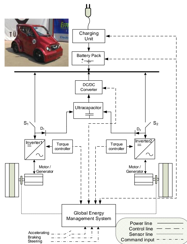
Fig. 1. General connection topology of Alalay-EV
