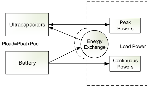
Fig. 2. General power sharing scheme [3]
