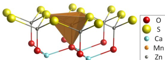
Fig. 1. Optimized structure of the Mn_{Zn} defect in CaZnOS.
