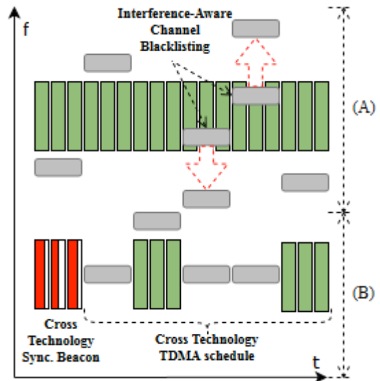
Figure 2 A basic (A) and advanced (B) cross-technology interference mitigation solution implemented using UPIs.
