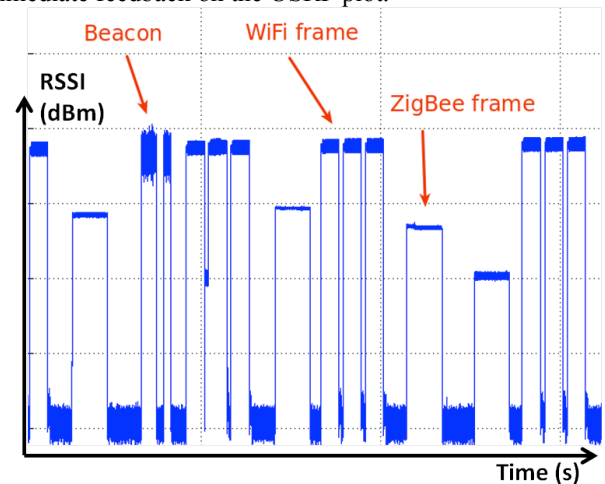
Figure 4 Live capture of RSSI (dBm) measured by the USRP over time.
