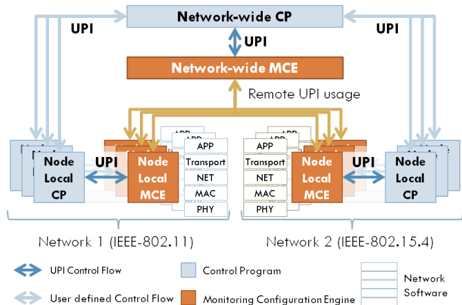
Figure 1 Conceptual overview of WiSHFUL control framework.
