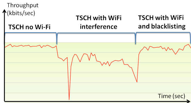
Figure 3 Live performance diagram showing the average network throughput (kbits/sec) over time.
