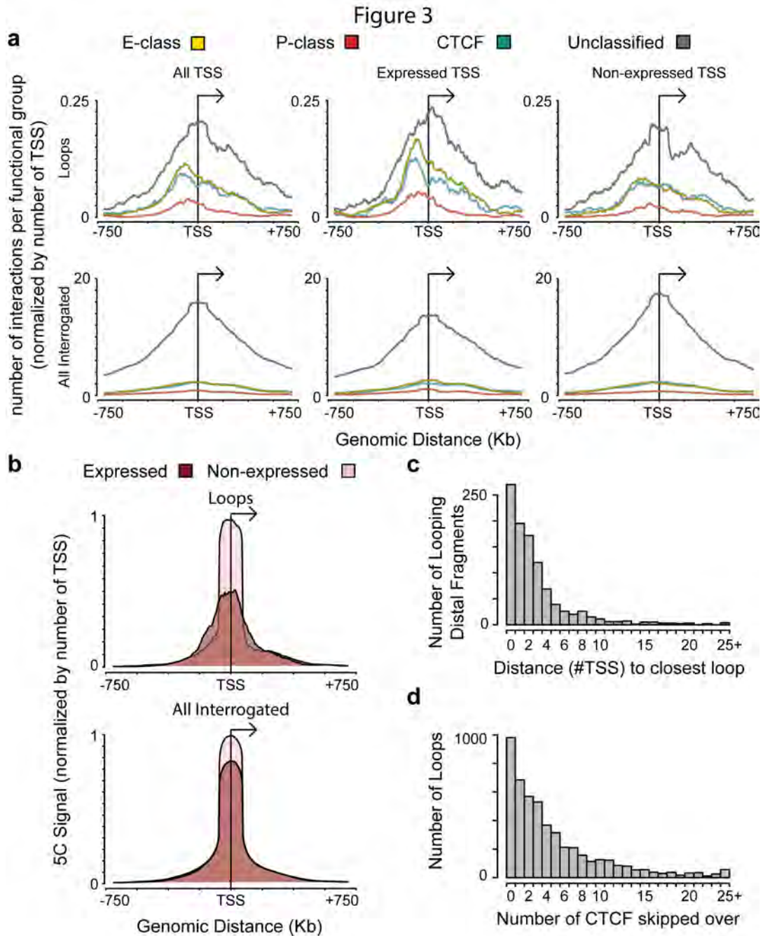
Figure 5.6 | Average looping landscape of TSSs to distal fragments. a, Composite profile of average number of group-specific looping interactions upstream and downstream of TSSs based on combined 5C interaction data from the four cell lines. Each group is represented by different colors. The top panel shows the average looping profiles of all TSSs (left), of expressed TSSs (CAGE
