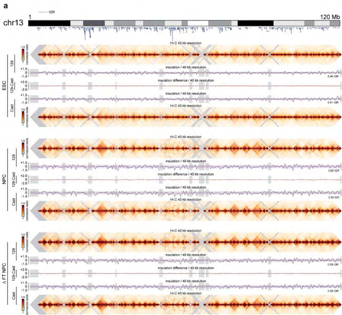
Figure 3.4 | chr13
