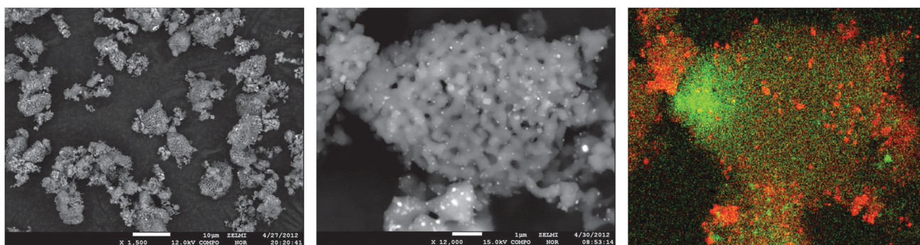
Fig. 4 SEM images of fresh Cat-2 ( Mn_xO_y-Na_2WO_4/SiO_2 ) and EDX-mapping of W L-edge (green) and Mn K-edge (red).
