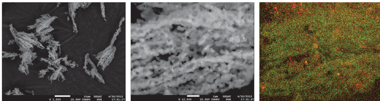
Fig. 3 SEM images of fresh Cat-1 ( Mn_xO_y-Na_2WO_4/SBA-15 ) and EDX-mapping of W L-edge (green) and Mn K-edge (red).
