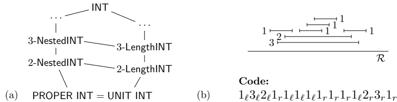
Figure 2 (a) The Hasse diagram of proper inclusions of the considered classes. (b) We can label each interval by the length of a maximal chain of nested intervals ending in it. We code the graph by the left-to-right sequence of left endpoints \ell and right endpoints r together with their labels.
