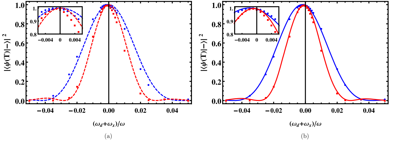
Figure 7. Fidelity |\langle \psi(T) | - \rangle|^2 against the deviation from resonant shaking (\omega_x + \omega_d)/\omega for V_0 = 3\hbar\omega and T = 300\omega^{-1} (resonant shaking corresponds to \omega_x = -\omega_d ). Polynomial scheme (red) and piecewise scheme with t_S = 0.75T (blue). Points correspond to the full Schrödinger equation, dashed lines to the 4-level model and lines to the 6-level model (B.2).
