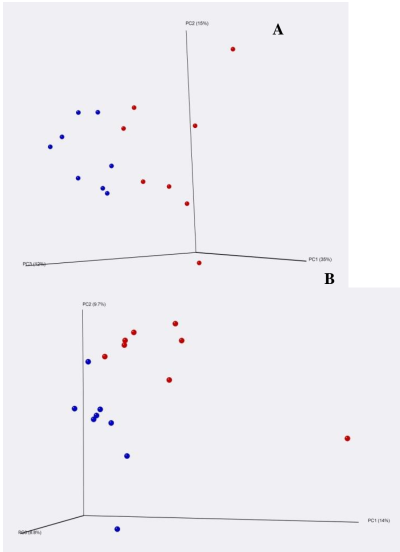
Figure 3.3 PCoA analysis based on weighted Unifrac (A) and unweighted Unifrac (B) distances; t 10 , c 12 CLA supplemented group (red circles) and unsupplemented group (blue circles); n=8 per group.
