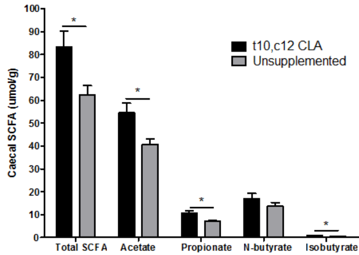
Figure 3.2 Caecal SCFA concentration in mice receiving a diet supplemented with t10, c12 CLA or with no supplementation; n=8 per group (Student t test; *p<0.05 )
