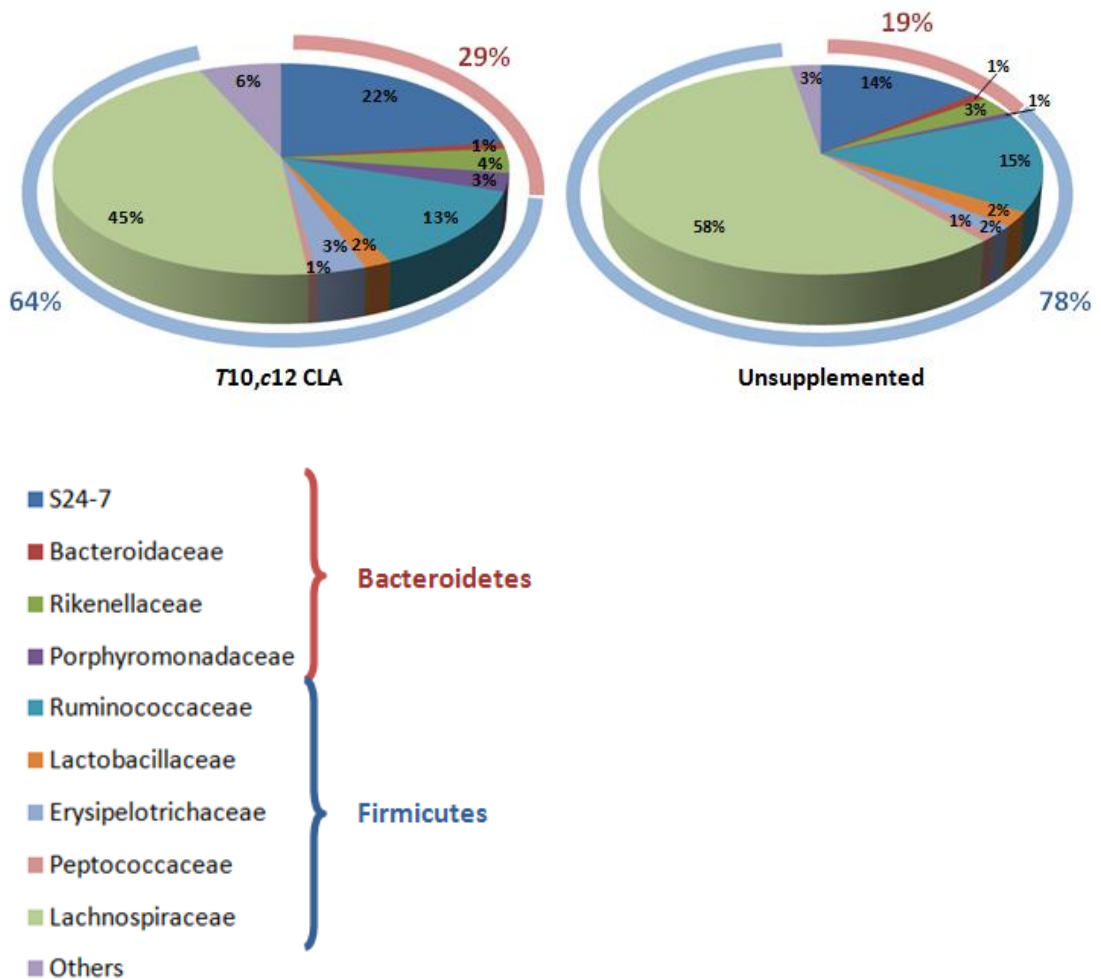
Figure 3.4 The gut microbiota composition is altered in mice receiving t10, c12 CLA supplementation, as determined by pyrosequencing of 16S rRNA (n=8 per group). Pie charts represent the mean percentage read number for the corresponding colour coded family (only reads \geq 1\% are shown).
