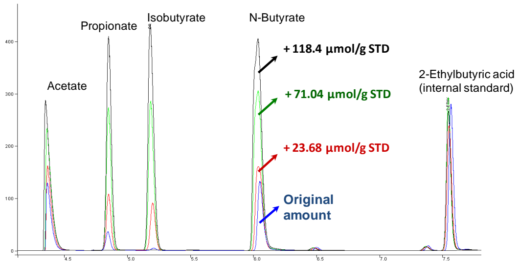
Figure 2.2 Recovery test overlaid chromatograms
