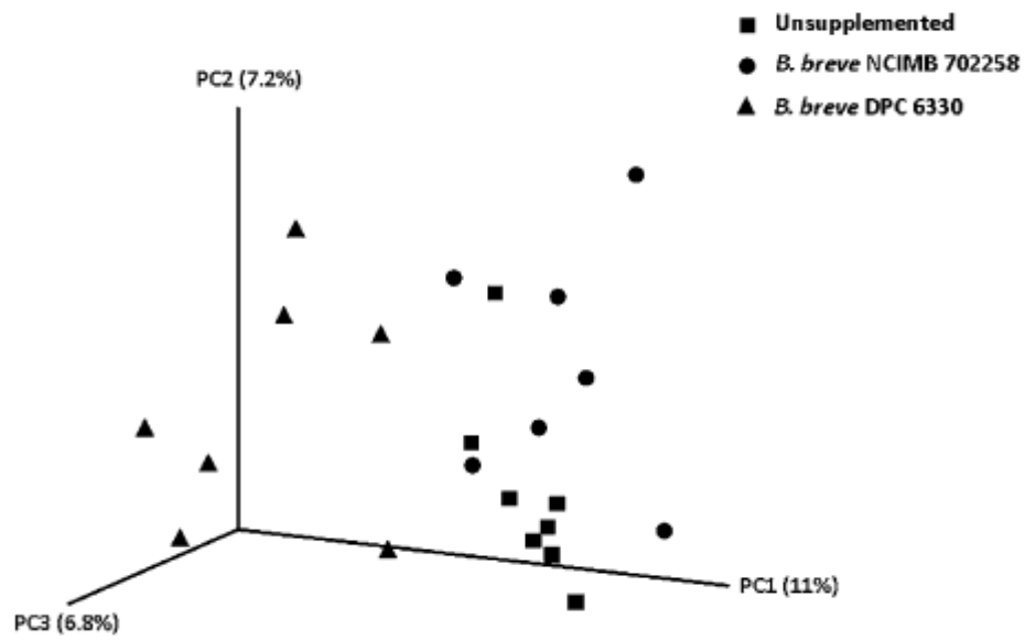
Figure 4.4 Principal coordinate analysis using unweighted UniFrac distances in mice supplemented with Bifidobacterium breve DPC 6330 (n=7) or B. breve NCIMB 702258 (n=7) and in unsupplemented mice (n=8).
