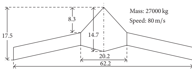
FIGURE 3: Planform of a flying wing aircraft model (unit: m).
