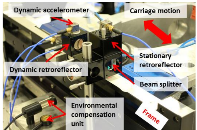
Fig. 7. Setup of the displacement validation experiment.
