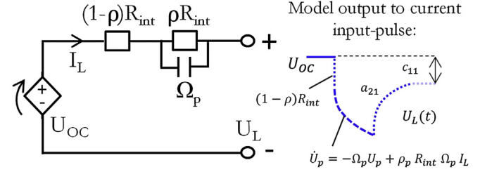
Fig. 3. Response of the Thevenin and behavioural battery model to a current pulse. (Details of the pulses used are given in Section 5).
