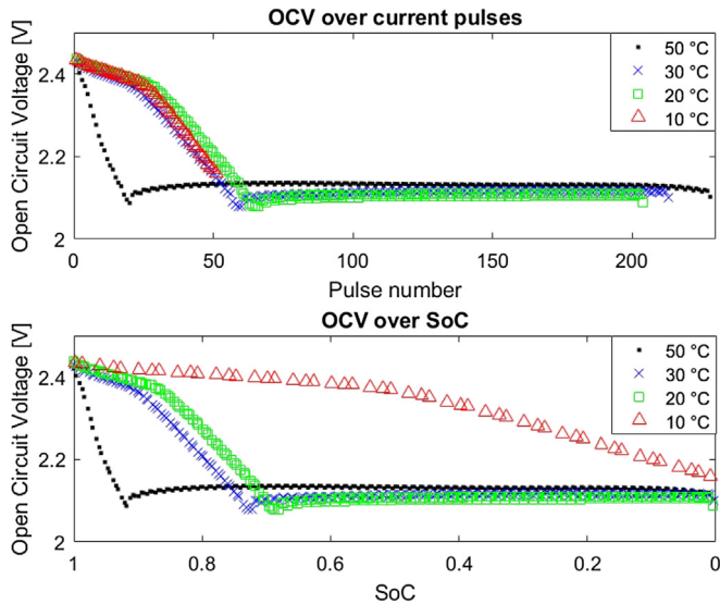
Fig. 5. Identification results for U_{OC} over Pulse and SoC.
