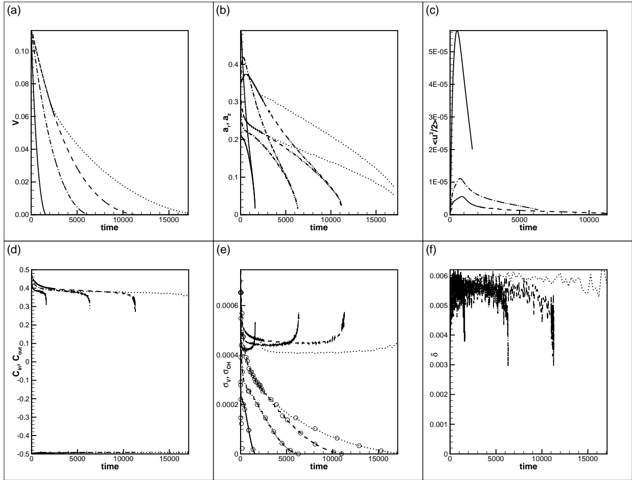
Figure 2: The droplet evolution at different Peclet numbers. The results are shown for A = -0.5 , H = 3 , r_0 = 0.3 , Gr = 0.1 , Ca = 2.5 \cdot 10^{-5} , Re = 10^3 , and Pe = 10^5 (solid line), Pe = 5 \cdot 10^5 (dash-dot line), Pe = 10^6 (dashed line). The dotted lines are obtained for the run with neglected convective flows (for Pe = 10^6 ). (a) Volume vs. time; (b) droplet's radius and length vs. time; (c) Kinetic energy averaged over the total volume of the tube vs. time; (d) Average concentrations in the droplet and in the surrounding solvent; (e) Surface tension coefficients vs. time, the lines marked by circles depict the curves of the surface tension calculated on the basis of the Vonnegut formula, \sigma_V , and the other curves show the surface tension coefficients calculated on the basis of the phase-field formula, \sigma_{CH} ; and (f) Interface thickness vs. time.
