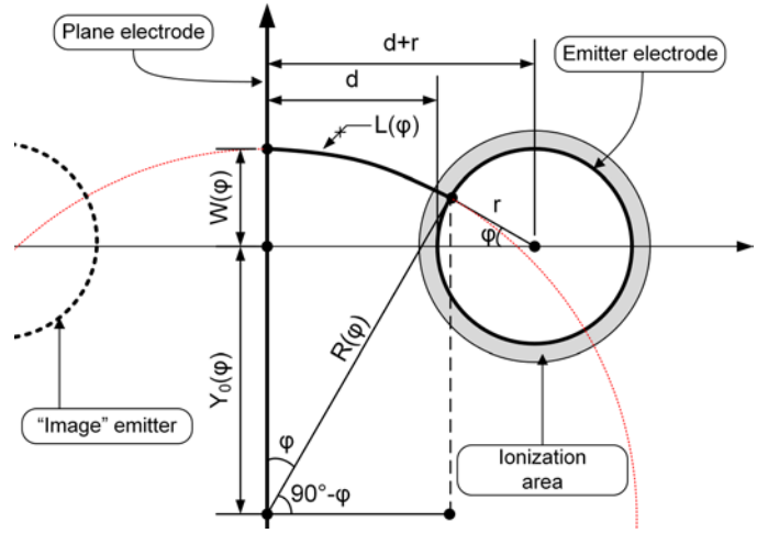
Fig. 1. Cylinder-plane electrode configuration and the formation of field lines.
