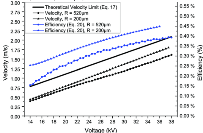
Fig. 15. Comparison of the EHD velocity and the efficiency for needle-grid configurations using two different grid collectors ( d = 4 \text{ cm} , r = 32 \mu\text{m} ).
