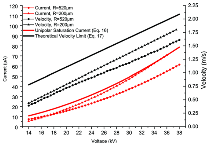
Fig. 14. Comparison of the EHD velocity and the corona discharge current according to (17) for needle-grid configurations using two different grid collectors ( d = 4 \text{ cm} , r = 32 \mu\text{m} ).
