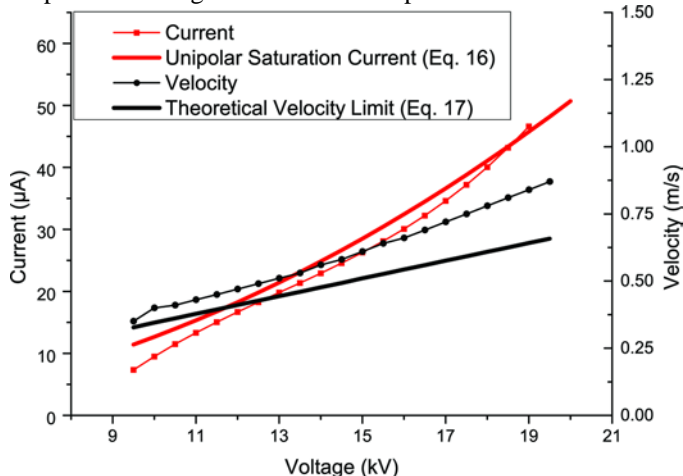
Fig. 13. Correlation between the corona current and the EHD velocity according to (17) for a needle-grid configuration of d = 2 \text{ cm} , r = 32 \mu\text{m} and R = 520 \mu\text{m} .
