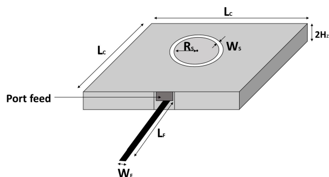
Fig. 1. Layout of the proposed antenna
