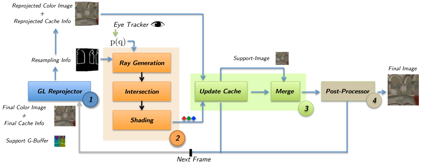
Figure 2: Building blocks of our reprojection pipeline. Old color and auxiliary cache info are reprojected using a GL Reprojector (Block 1). New rays are generated based on the user’s gaze and possible errors introduced by the reprojection are marked in a resampling info buffer. The ray traced pixel values (Block 2) are blended using a temporal caching and merging scheme (Block 3). An optional Post-Processor is used to smooth artifacts arising from stochastic sampling processes like ambient occlusion (Block 4).
