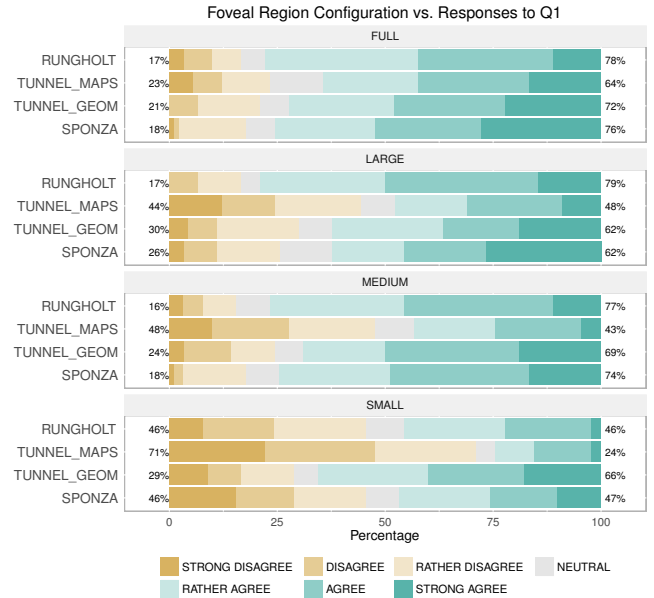
Figure 7: Likert-scale ratings for Q1 (Has the shown sequence been free of visual artifacts?) for all scenes grouped by foveal region configurations. The percentages on the left and right represent the fraction of all participants that had a tendency towards disagree and agree , respectively. As clearly visible, the smallest foveal region configuration revealed a significant amount of artifacts, while the larger foveal regions were close to the full renderer in this regard.
