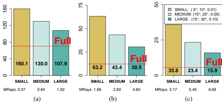
Figure 5: Influence of configuration of the foveal regions on FPS for the scene Sponza, rendered with a point light source (a), an area light source with 8spp (b) and with ambient occlusion with 16spp (c). MRays denotes the mean number of rays per frame. The scene was rendered at a resolution of 1182 \times 1464 using a NVIDIA GeForce Titan X.
