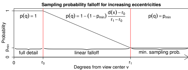
Figure 3: Probability p(q) for sampling a specific pixel q based on its eccentricity and user-defined parameters r_0 , r_1 and p_{min} . Despite the hyperbolic falloff of cones towards outer regions a linear falloff is employed to improve motion perception in the periphery and to reduce spatial and temporal aliasing artifacts in these areas.
