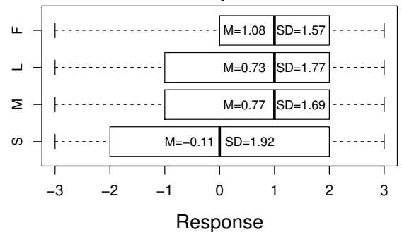
Figure 6: Likert-scale ratings of perceived visual artifacts for Small, Medium, Large, and Full foveal regions. While small caused neutral ratings on average, ratings for medium and large were not significantly different from full rendering (cf. Section 4.2.2, RQ1).
