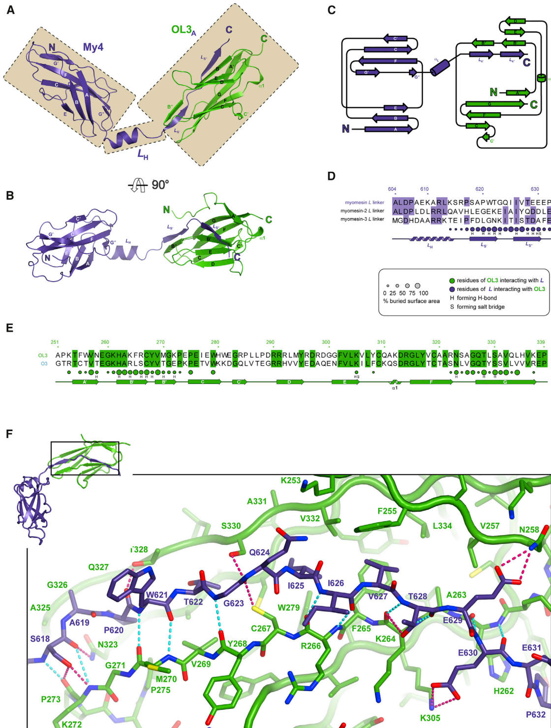
Figure 3. OL3:My4L Heterodimer
