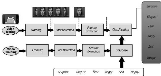
Figure 1: Overview structure of the facial expression recognition.
