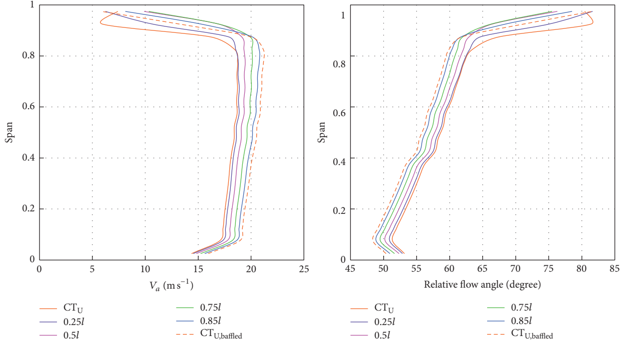
FIGURE 16: The distribution of inlet velocity for different baffle lengths at m = 3.4 kg/s.
