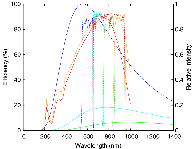
Figure 2. Andor iKon-M 934N BR-DD quantum efficiency curve ( T_{\text{CCD}} = 25^{\circ}\text{C} solid orange, T_{\text{CCD}} = -90^{\circ}\text{C} solid red) over-plotted with the blackbody emission curves of a K0, K9 and M4.5 star and the NGTS custom bandpass filter set (dotted blue, cyan, green, orange, and red lines). Peak emission wavelengths (558, 784 & 967 nm for K0 (solid blue), K9 (solid cyan), and M4.5 (solid green) stars, respectively) for these stellar classes are well matched to the sensitivity of the DD-CCDs. The intensities given by Planck’s energy distribution equation have been scaled to 1 for clarity.
