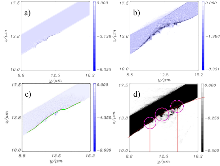
Fig. 4. Spatial distribution of the electron density profile on the target during the laser pulse at a) t = 5.3 fs, b) t = 32 fs and c) t = 21.3 fs from the start of the interaction for laser intensity 10^{21} W/cm 2 . Colour scales are normalized on the initial electron density ( 8 \times 10^{23} cm -3 ), and it shown negative because it is electron charge density. d) t = 21.3 fs at the normalization of electron density to 3 \times 10^{23} cm -3 .
