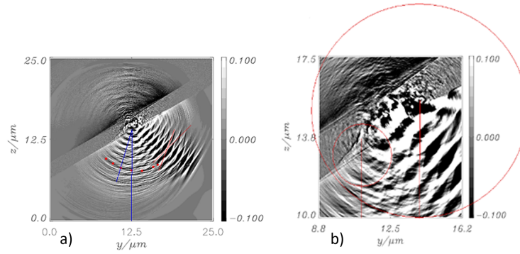
Fig. 5. a) 2D distribution of incident and reflected laser fields ( E_y component) at 42 fs of laser interaction in the whole box of simulation. Scales are normalized to the incident laser amplitude. b) Zoomed 2D distribution of incident and reflected fields at 42 fs of laser interaction. The centers of spherical secondary waves are shown in c). Incident laser intensity is 10^{21} W/cm ^2 .
