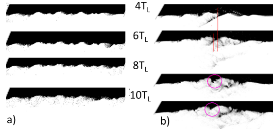
Fig. 6. The electron density profiles are depicted for integer number of laser periods: 4T_L, 6T_L, 8T_L, 10T_L for laser intensities a) 10^{19} W/cm 2 and b) 10^{21} W/cm 2 . Pulse duration 30 fs, 30° incidence, at the beam diameter 4 μm, size on the target 8.5 μm.
