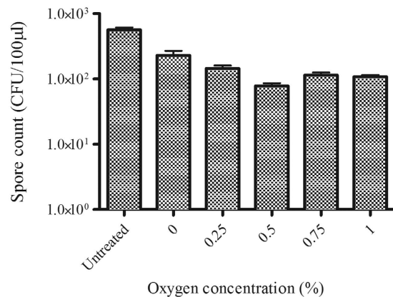
Figure 2. Survival of C. difficile spores after 60 seconds plasma exposure using varying oxygen concentrations within a helium plasma alongside untreated spores. Each bar represents the average of five replicates with error bars showing the standard error.
