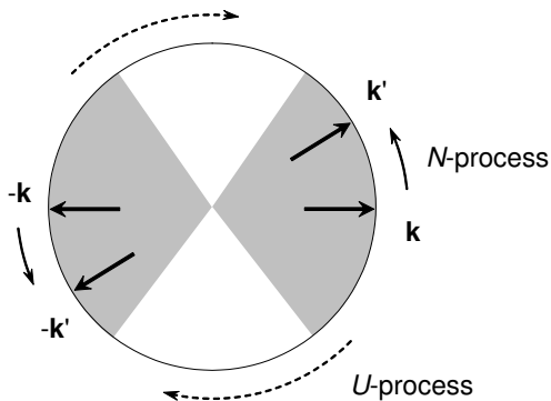
FIG. 8: Schematic of a spherical Fermi surface and a pair of electrons with initial states \mathbf{k} and -\mathbf{k} . The end states, \mathbf{k}' and -\mathbf{k}' , can be accessed via both normal ( N ) and umklapp ( U ) scattering, with different pair occupation probabilities, causing a dilemma.
