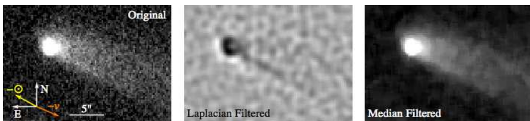
Figure 3. Enlarged versions of the near-nucleus tail structure from the R-band stack shown in Fig. 2. The original image (left) is shown together with versions processed using Laplacian (centre) and median (right) filters. A trail of larger particles leaving the nucleus and trailing the comet's orbital motion is visible in the Laplacian-filtered image. The median-filtered image highlights the near-nucleus part of the tail which points in the projected antisolar direction.
