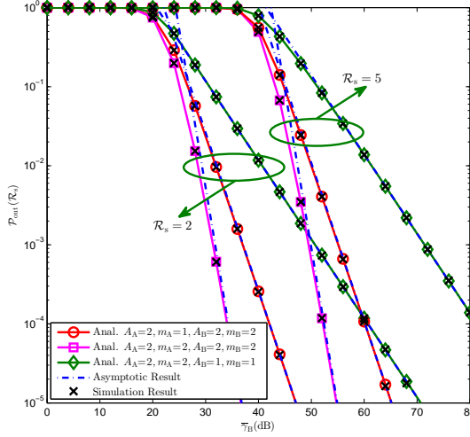
Fig. 2: Secrecy outage probability versus \bar{\gamma}_B for colluding eavesdropping with N_B=2 , N_E=A_E=m_E=2 , \gamma_T=20 dB and \bar{\gamma}_E=5 dB.
