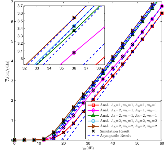
Fig. 6: Ergodic secrecy rate versus \bar{\gamma}_B for colluding eavesdropping with N_B=2, N_E=m_E=A_E=2, \gamma_T=30 dB and \bar{\gamma}_E=10 dB.
