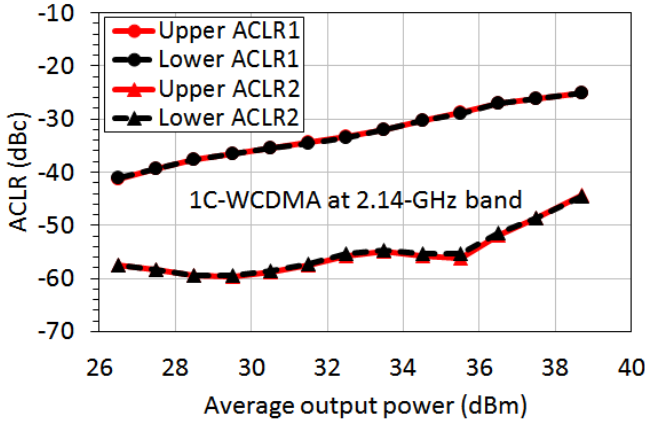
Fig. 26. Measured ACLRs against the average output power with single carrier 5-MHz W-CDMA signal at 2.14 GHz with 6.5-dB PAPR. ACLR 1 and ACLR 2 are at 5- and 10-MHz offsets from the carrier frequency, respectively.
