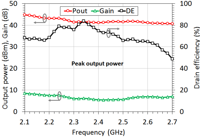
Fig. 21. Measured output power, gain and DE versus frequency at PP level with V_{gM} = -2.7 V, V_{gA} = -4.75 V and V_{dc} = 28 V.
