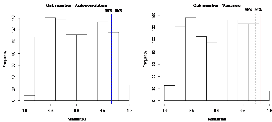
Figure 5: Histograms showing the Kendall tau distribution of 1000 randomised iterations of the original data for a) autocorrelation and b) variance. The black dotted lines show the 90% and 95% significance levels and the blue and red lines indicate the Kendall tau values from analysis on the original data, with corresponding p values of <0.1 and <0.01 for autocorrelation and variance respectively.
