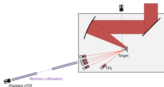
Figure 1: Experimental setup
