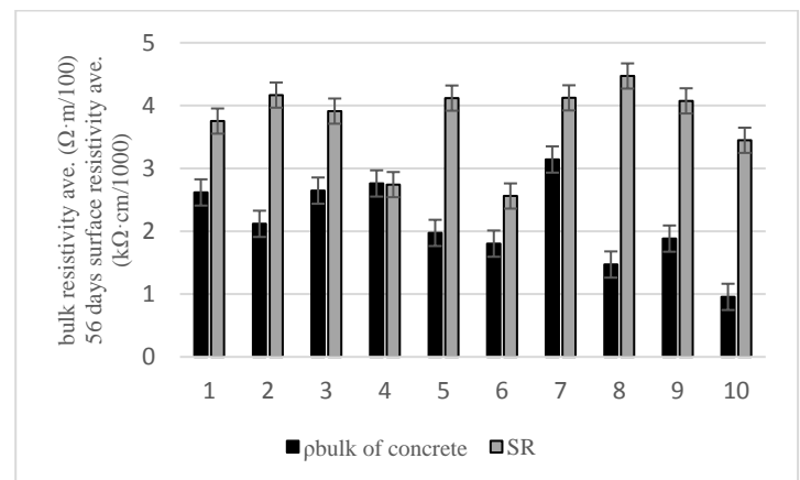
Figure 8 bulk and SR of the AAS concrete mixes
