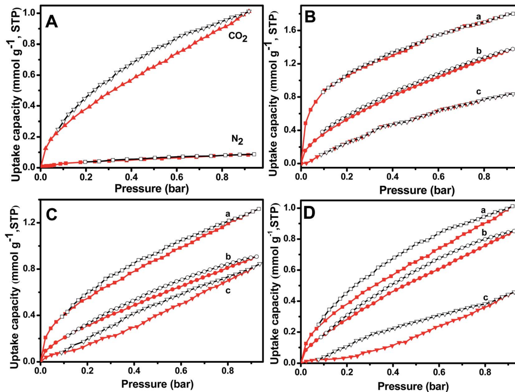
Fig. 6 \text{N}_2/\text{CO}_2 isotherms (adsorption branch in red and desorption in black) of sample NPC-723 at 293 K (A) and \text{CO}_2 isotherms of samples NPC-723 (a), NPC-873 (b) and NPC-1173 (c) at different temperatures: 253 K (B), 273 K (C) and 293 K (D).
