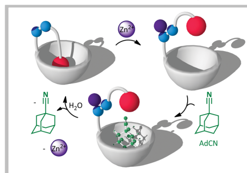
Scheme 9 A zinc(II)-ion switchable cavitand 11 .
