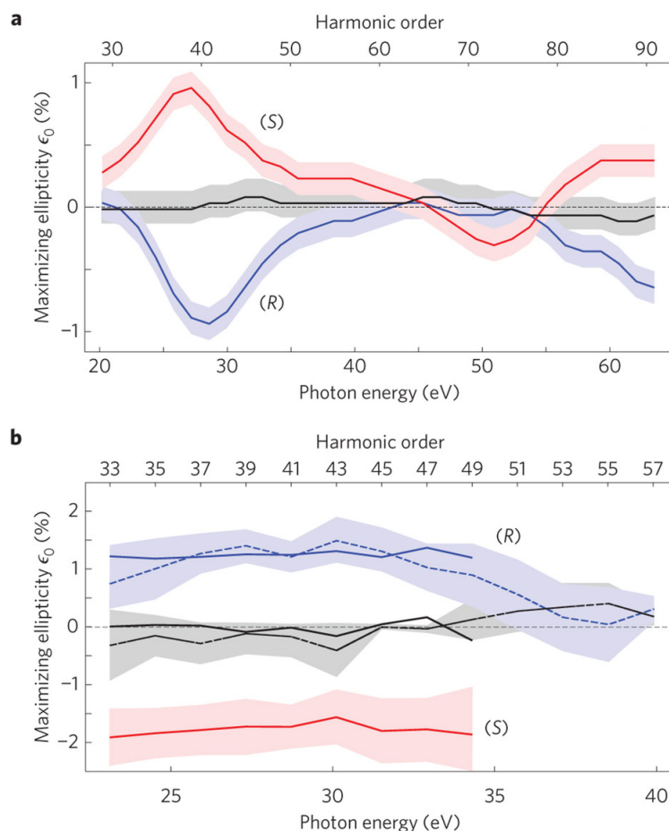
Figure 9. Maximizing ellipticity as a function of the harmonic order for epoxypropane (a) and fenchone (b), where red and blue traces correspond to S- and R-enantiomers, respectively. The grey line represents the non-chiral reference. From [69] with permission.
