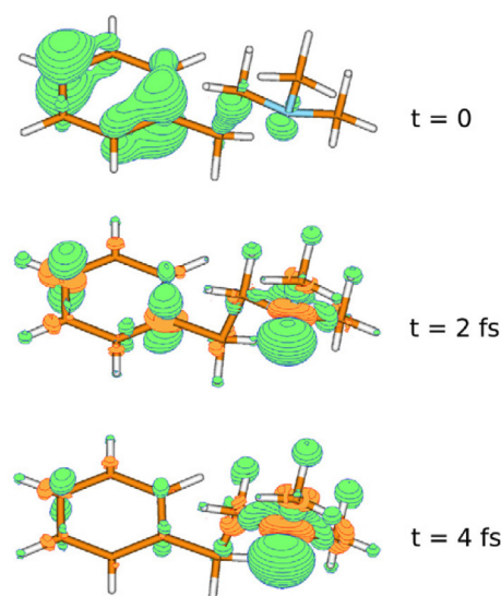
Figure 4. Time evolution of the 3D-hole density of PENNA calculated for the geometry with the C_1 - C_2 bond elongated by 20 pm. Adapted from [59].
