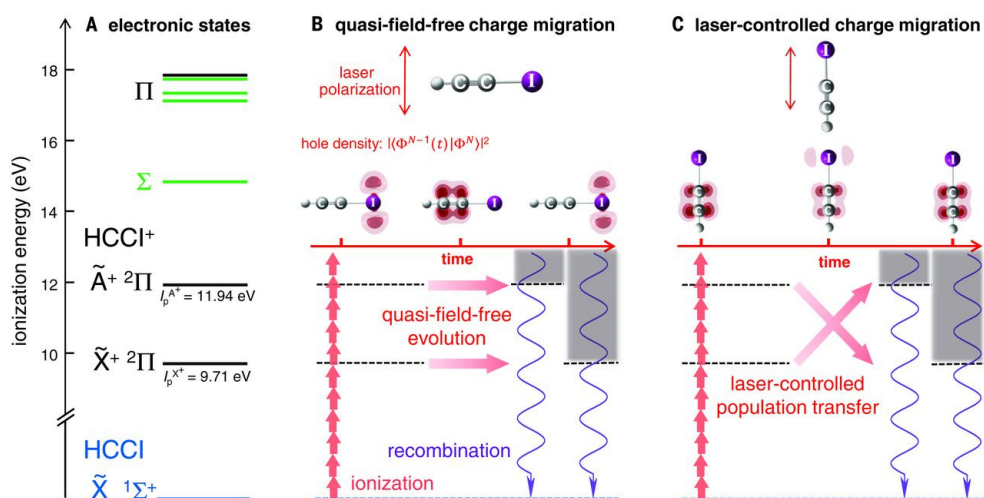
Figure 10. (a) Electronic states of \text{HCCI}^+ . (b) Quasi-field-free charge migration and (c) laser controlled charge migration induced in iodoacetylene molecule, when the molecule is aligned perpendicular (b) and parallel (c) with respect to the laser polarization axis. From [51] with permission.
