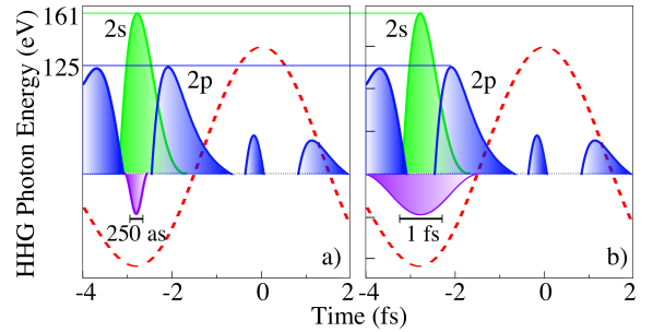
FIG. 3: (Color online) The maximum emitted harmonic photon energies that would result from electrons being released at the times shown along the horizontal axis for both 2p (blue) and 2s (green) electrons from Ne in a 18 fs, 1.8 \mu\text{m} , 1.2 \times 10^{14} \text{ Wcm}^{-2} pulse (red dashed line). Trajectories are initiated by a a) 250 as and b) 1 fs 45 eV XUV pulse. Trajectories of 2s and 2p which lead to recollision are localized in time, and therefore can be resolved in the short-pulse case (a). For a long XUV pulse (b), both electrons contribute.
