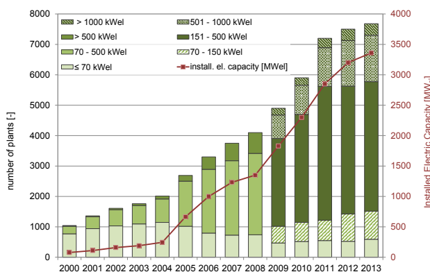
Growth of Biogas Plants in Germany Source: IEA Bioenergy Germany 2014:15
