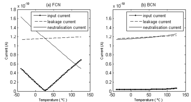
Fig. 6 Temperature corner sweep of (a) FCN. (b) BCN.
