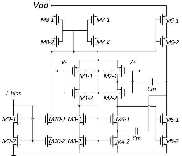
Fig. 1 Circuit of (a) back-gate current neutralisation FEA. (b) Drain voltage generation circuit.
