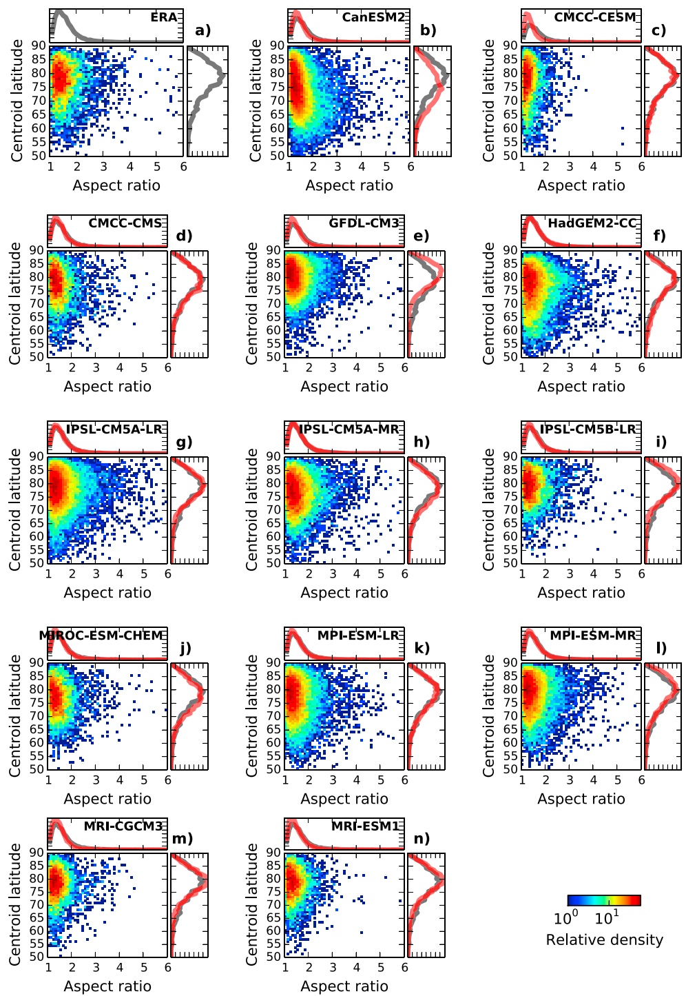
Figure 2. (a–n) Distributions of centroid latitude (y axis) and aspect ratio (x axis) for ERA-40/I (Figure 2a and grey lines in Figures 2b–2n) and the CMIP5 models (Figures 2b–2n; red lines). Joint distributions are shown with a logarithmic scale such that red squares represent the densest regions.
