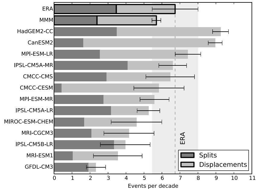
Figure 3. Frequency of split and displaced vortex events in the CMIP5 models, ERA-40/I, and the multimodel mean (MMM). Error bars are for the frequency of all events and represent 1σ range, assuming a binomial distribution of events. The grey shaded region represents the 1σ range for ERA-40/I, along with the mean (dashed line).
