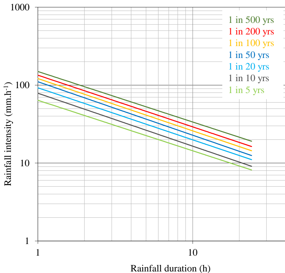
1 2 Figure 3: Rainfall Intensity Duration Frequency curves for Saint Lucia developed by Klohn-Crippen (1995) using Gumbel analysis 3 of 40 years of hourly rainfall data from 15 rainfall gauges.
