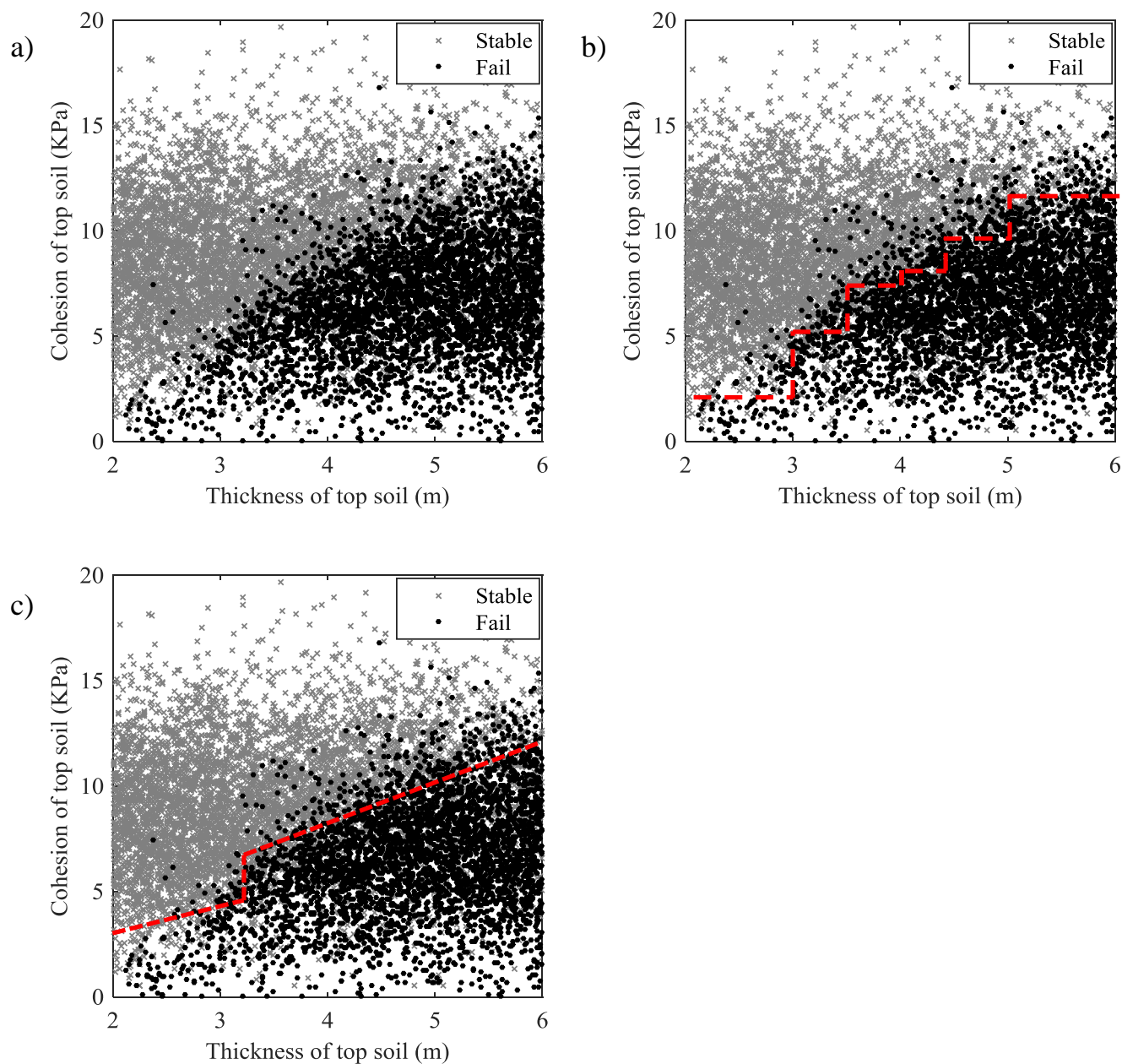
1 2 Figure 6: a) Sampled values of effective cohesion of top soil versus thickness of top soil. Black points correspond to simulations 3 resulting in slope failure, while grey crosses correspond to simulations resulting in a stable slope. b) Same as panel a, with the 4 additional red dashed line representing the thresholds derived from the classification tree in Fig. 5. c) Same as panel a, with the 5 additional red dashed line representing the thresholds derived from the classification tree in Fig. 9.
