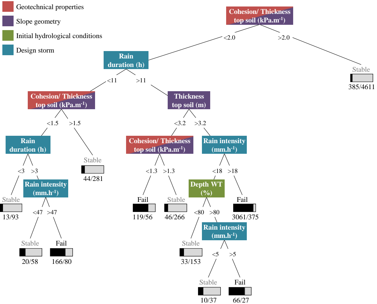
2 Figure 7: Classification tree of slope response, when adding an auxiliary variable (ratio between effective cohesion and thickness of 3 top soil) among uncertain input factors. The bar under each leaf shows the proportion and total number of simulations leading to 4 slope failure (black bar, left hand number) or a stable slope (grey bar, right hand number).
