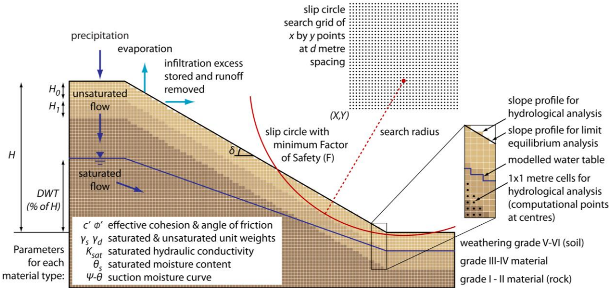
1 2 Figure 2: Conceptual model of the experimental slope. CHASM uses the Bishop method of slices to perform slope stability analysis, 3 which involves a numerical search for the slip surface.
