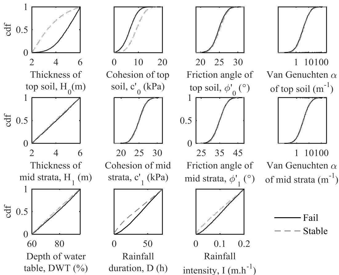
1 2 Figure 4: Cumulative probability distributions (cdf) of slope failure and stability predicted by CHASM for several different input 3 factors. Note that the Van Genuchten suction-moisture curve \alpha is shown in logarithmic scale.
